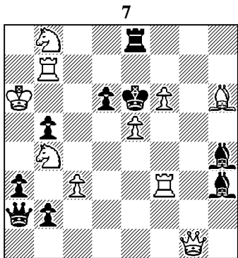
Mate in 2 moves (10+9)
