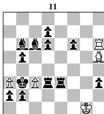
Helpmate in 3 moves (5+12) 3 solutions
