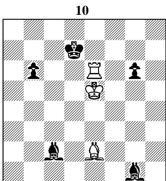
White to move and win (3+5)
