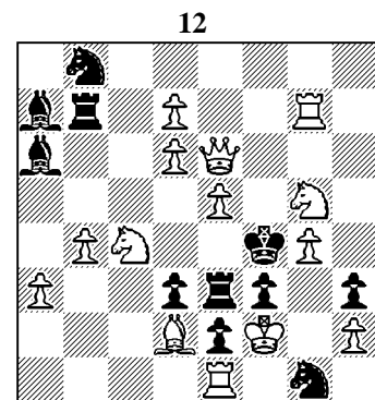
Selfmate in 5 moves (14+11)
