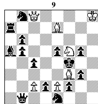
Mate in 4 moves (7+14)
